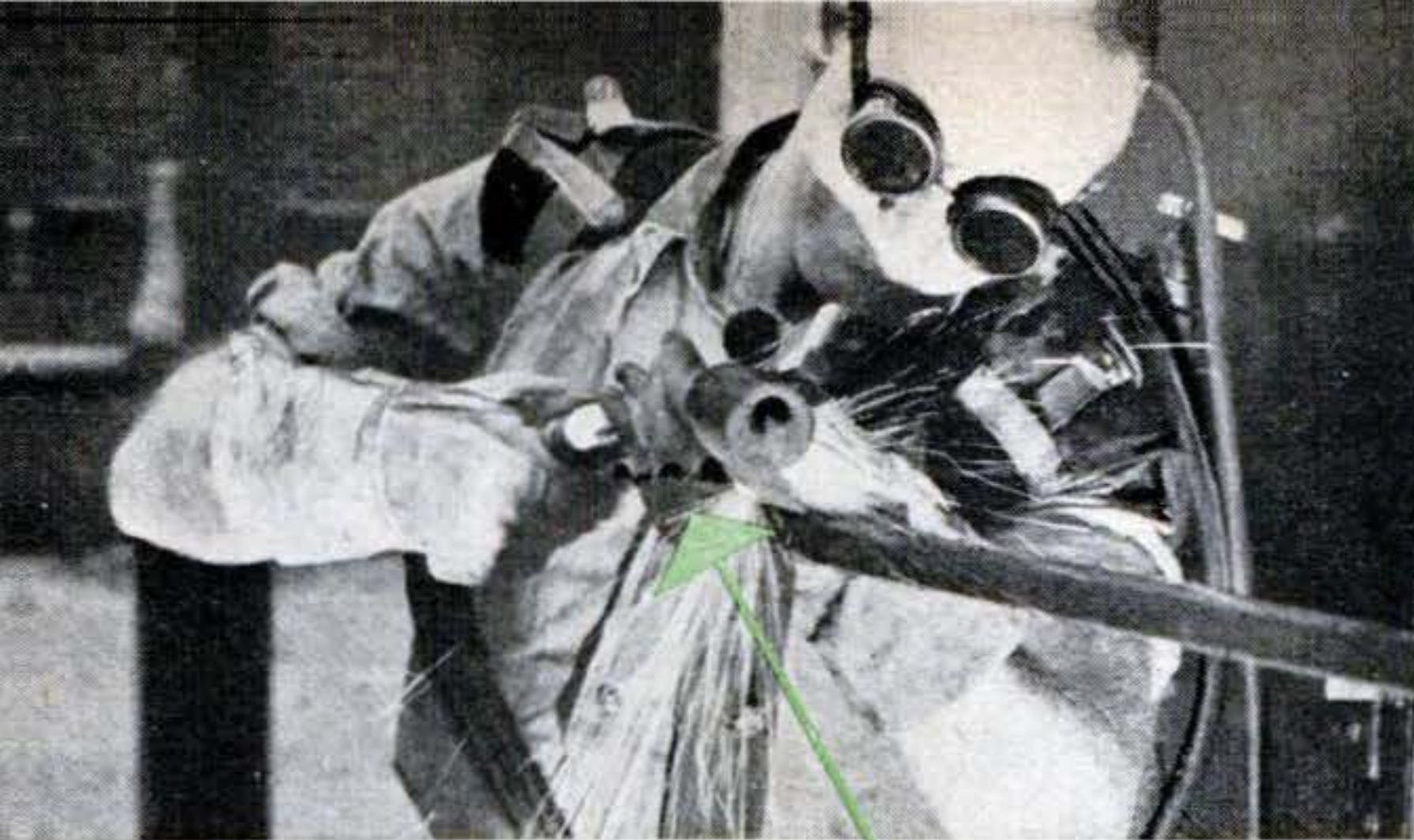
OXYACETYLENE TORCH is used to free people caught between elevators and shafts and to cut steel girders. Danger of igniting gasoline bars its use in auto-wreck rescues.
